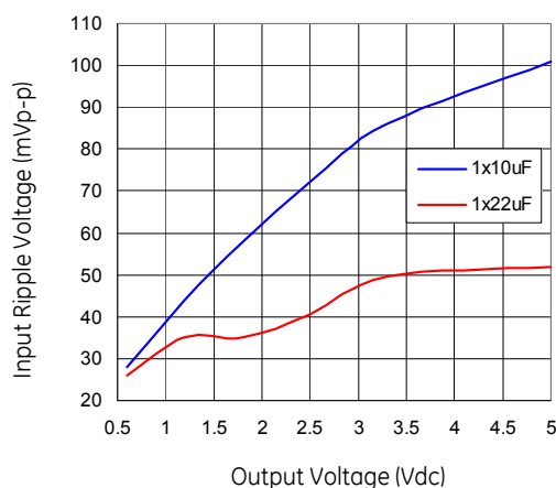
Figure 41. Input ripple voltage for various output voltages with 1x10 \mu F or 1x22 \mu F ceramic capacitors at the input (2A load). Input voltage is 12V.
