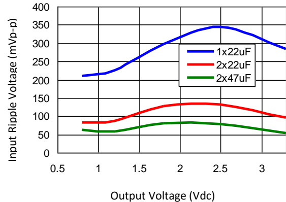
Figure 28. Input ripple voltage for various output voltages with 1x22 μF, 2x22 μF or 2x47 μF ceramic capacitors at the input (30A load). Input voltage is 12V.
