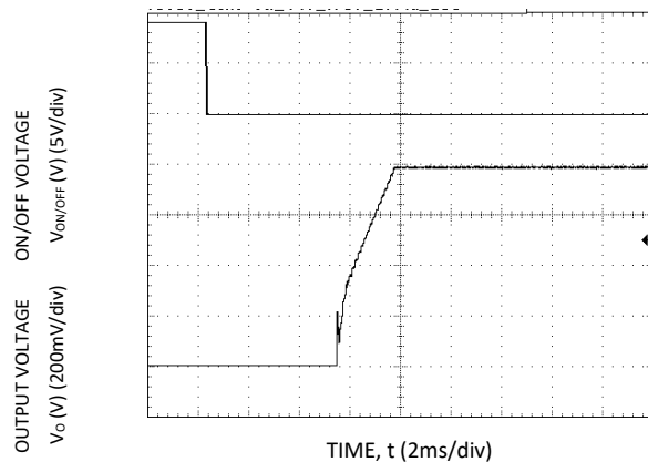
Figure 3. Typical Start-up Using On/Off Voltage ( I_o = I_{o,max} ).
