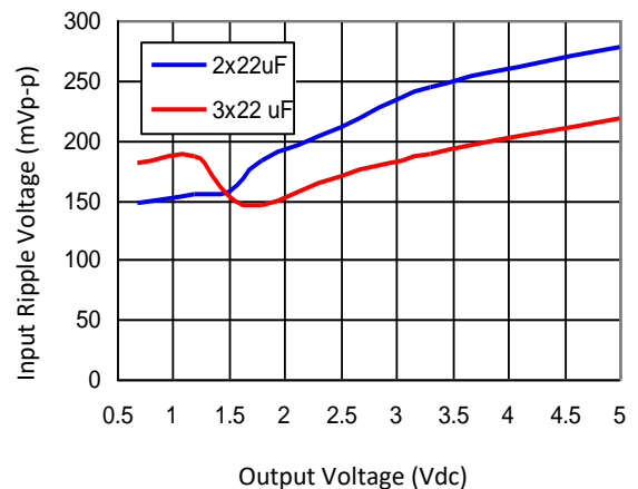
Figure 40. Input ripple voltage for various output voltages with 2x22 \mu F or 3x22 \mu F ceramic capacitors at the input (20A load). Input voltage is 12V.
