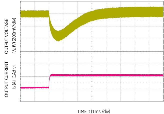
Figure 16. Transient Response to Dynamic Load Change from 50% to 100% at 12Vin, C_{out}=9\times 10\mu\text{F} , C_{Tune}=3300\text{pF} , R_{Tune}=30.1\text{k}\Omega
