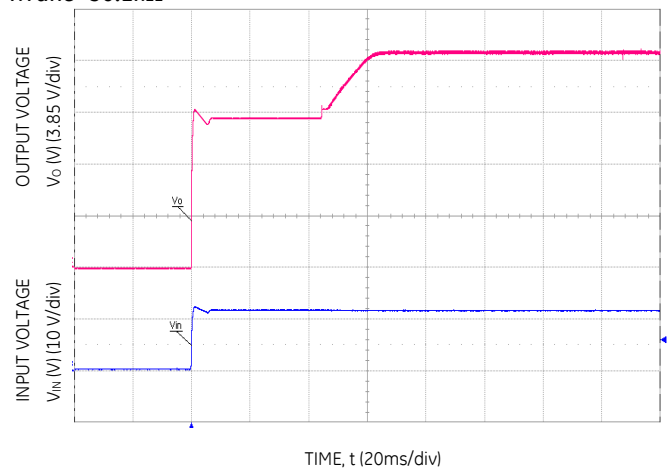
Figure 6. Typical Start-up Using Input Voltage ( V_{in}=12\text{V} , I_o=I_{o,max} ).
