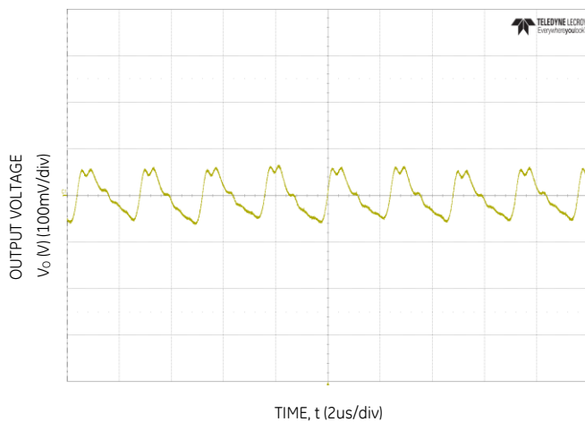
Figure 21. Typical output ripple and noise ( C_o=66\mu\text{F} ceramic, V_{IN} = 12\text{V} , I_o = I_{o,max} ).
