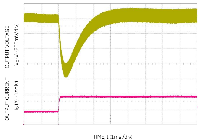
Figure 22. Transient Response to Dynamic Load Change from 0.9A to 1.9A at 12Vin, C_{out}=9\times 10\mu\text{F} , C_{Tune}=1000\text{pF} , R_{Tune}=30.1\text{k}\Omega
