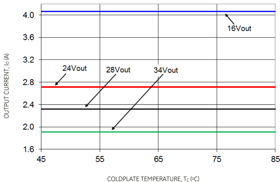
Figure 34. Output Current versus Coldwall Temperature; V_{IN} = 12\text{V} .
