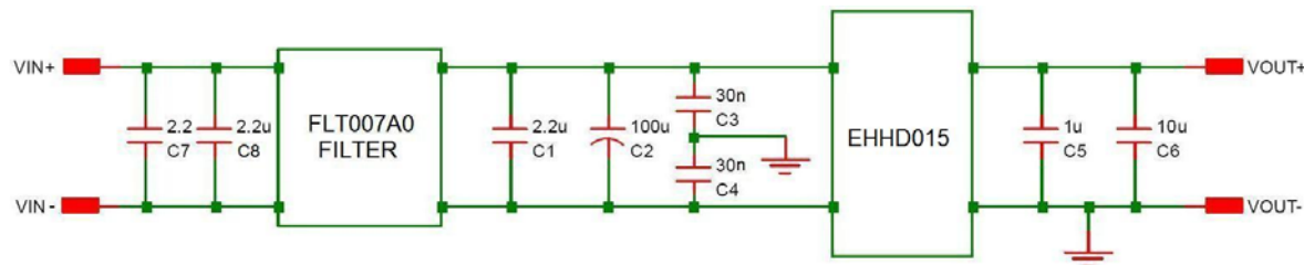
Figure 29. EMC Considerations
