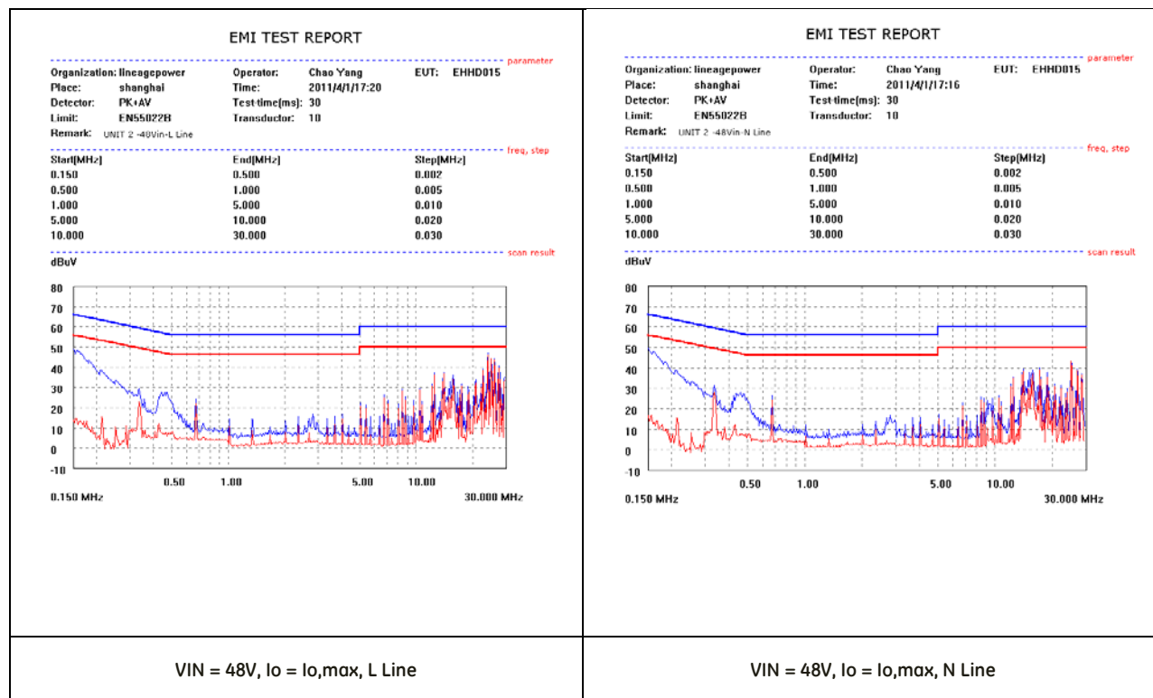
Figure 29. EMC Considerations
