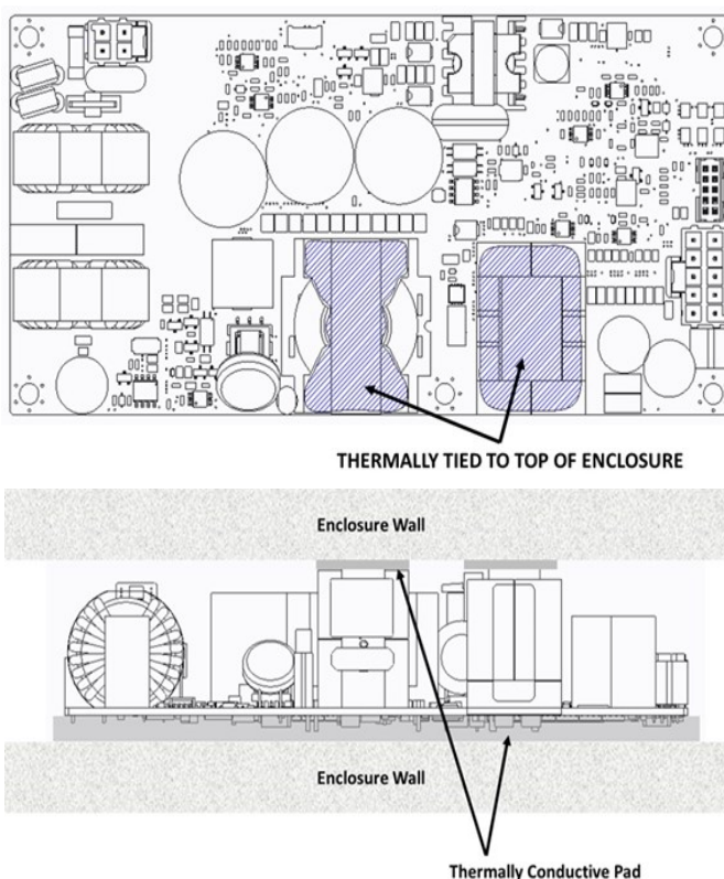
Fig. 3. Example of the CLP0612DC for sealed enclosure applications
