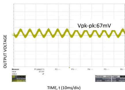
Figure 2. Typical output ripple and noise ( V_{in} = 230V_{ac} , load).
