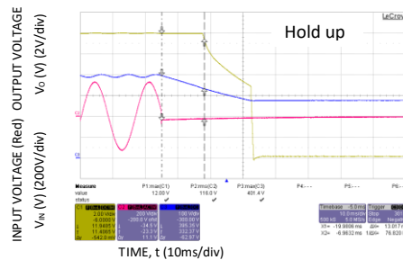
Figure 7. Typical Hold-up waveforms ( V_n = 230V , 100% Load).
