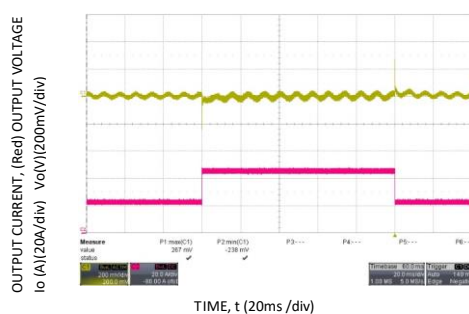
Figure 3. Transient Response to Dynamic Load change 100% from 50% to 100% at V_{in} = 230V_{ac} .
