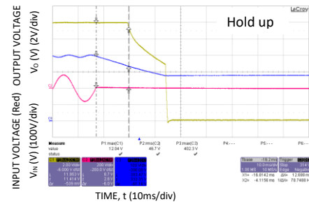
Figure 6. Typical Hold-up waveforms ( V_n = 115V , 100% Load).
