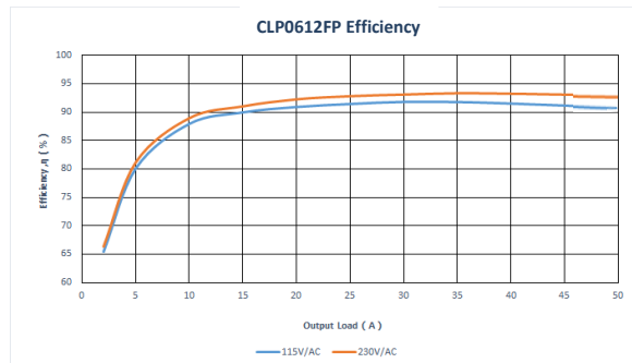
Figure 1. Power Supply Efficiency versus Output Current
