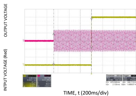
Figure 4. Typical Start-up ( V_{in} = 90V_{ac} , Full Load).
