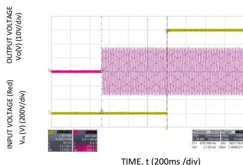
Figure 5. Typical Start-up ( V_{in} = 230V_{ac} , Full load).
