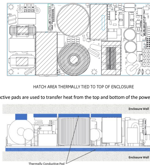
Fig. 1. Example arrangement of the CLP0612 for sealed enclosure applications.
