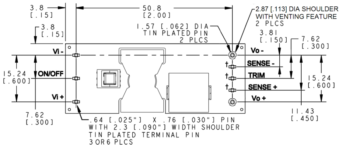
Bottom View
