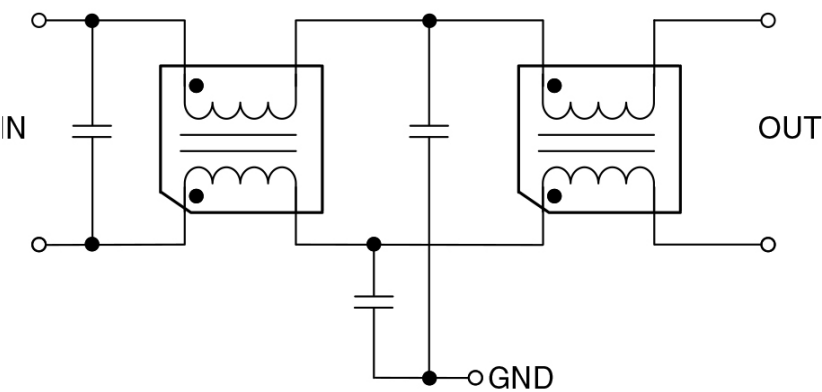
Figure 5. Internal Schematic
