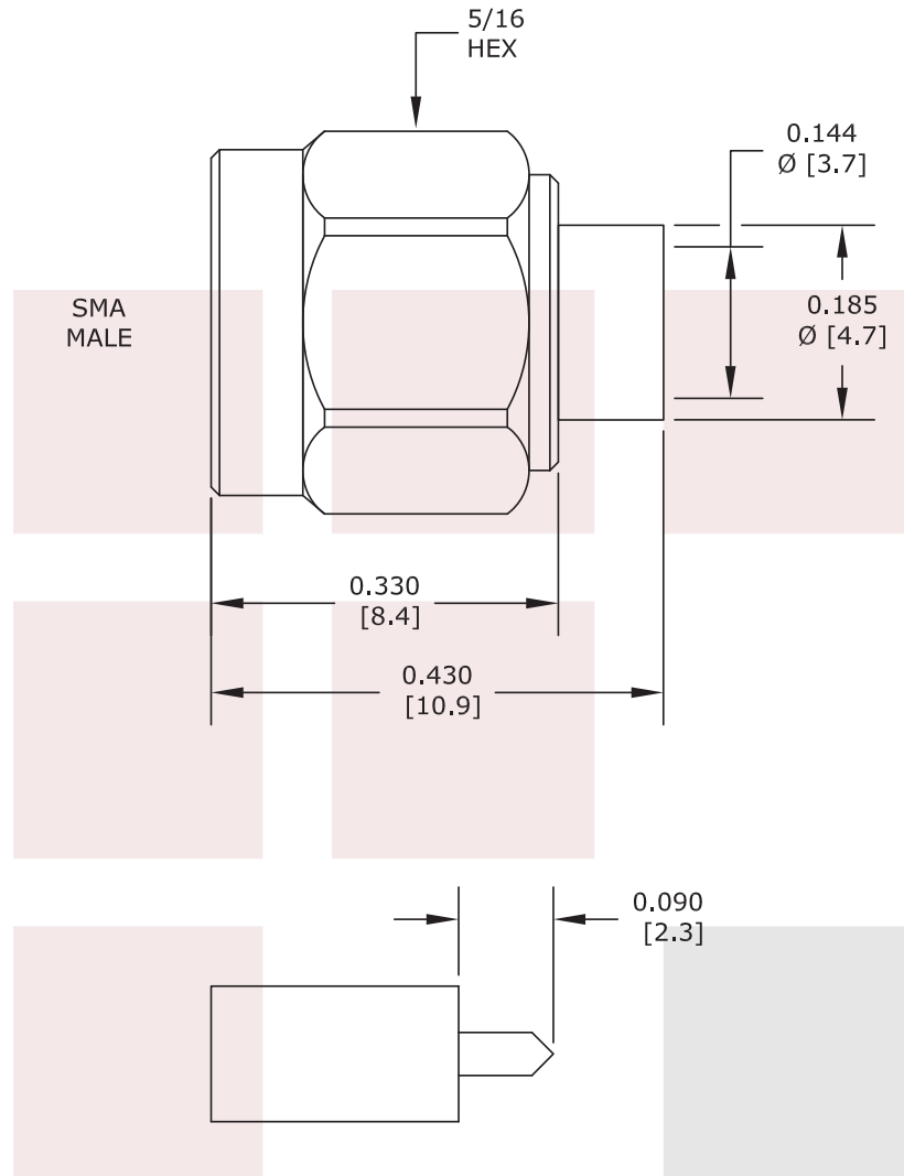
STRIPPING DIMENSIONS
