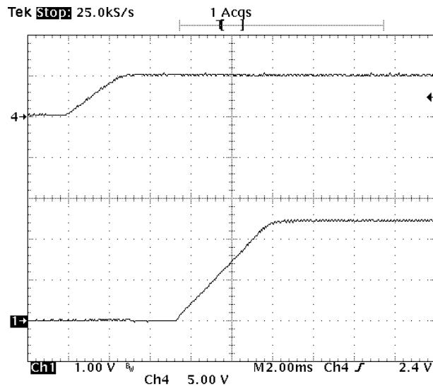
Fig-2.5V-4: Turn-on transient for V_{out}=2.5V with application of V_{in} at full rated load current (resistive) and 47\mu F \times 4 external capacitance at V_{in}=5.0V .
