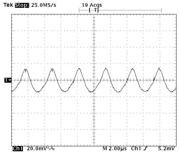
Fig-0.7525V-5: Output voltage ripple (20mV/div.) for V_{out}=0.7525V at full rated load current into a resistive load with external capacitance 47\mu F \times 4 ceramic + 1\mu F ceramic at V_{in}=5.0V .
