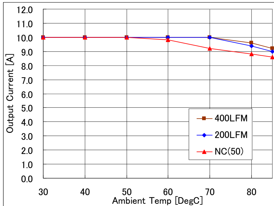
Fig-2.5V-1: Available load current vs. ambient temperature and airflow rates for Vout=2.5V with Vin=5.0V. Maximum component temperature \leq 120^{\circ}\text{C}
