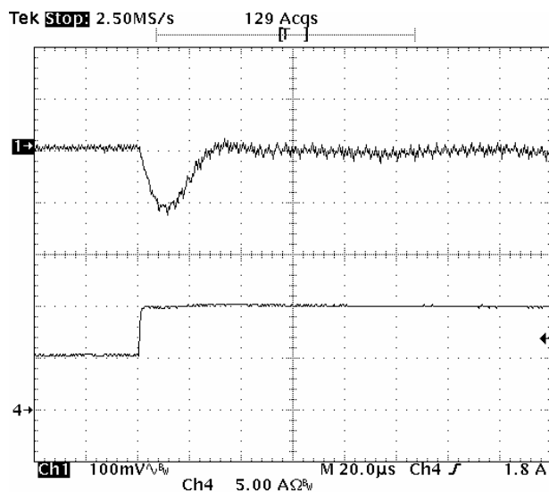
Fig-2.0V-6: Output voltage response for V_{out}=2.0V to positive load current step-change from 5A to 10A with slew rate of 5A/\mu s at V_{in}=5.0V . C_o=47\mu F \times 4 ceramic + 1\mu F ceramic.
