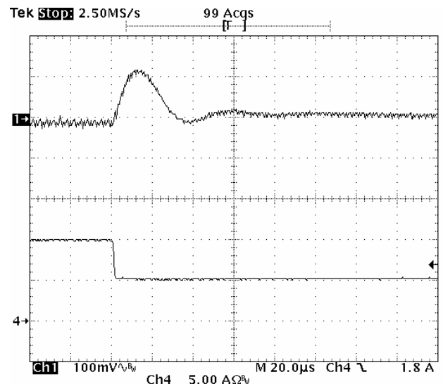
Fig-1.2V-7: Output voltage response for V_{out}=1.2V to positive load current step-change from 10A to 5A with slew rate of -5A/\mu s at V_{in}=5.0V . C_o=47\mu F \times 4 ceramic + 1\mu F ceramic.
