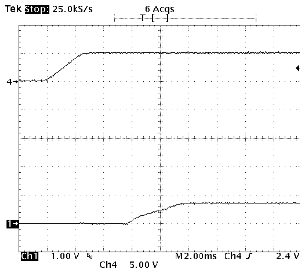
Fig-0.7525V-4: Turn-on transient for V_{out}=0.7525V with application of V_{in} at full rated load current (resistive) and 47\mu F \times 4 external capacitance at V_{in}=5.0V .
