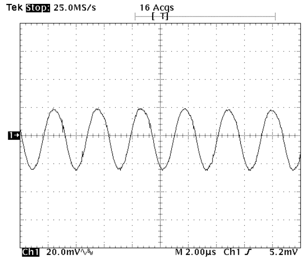
Fig-2.5V-5: Output voltage ripple (20mV/div.) for V_{out}=2.5V at full rated load current into a resistive load with external capacitance 47\mu F \times 4 ceramic + 1\mu F ceramic at V_{in}=5.0V .
