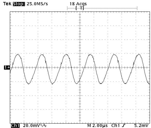
Fig-1.5V-5: Output voltage ripple (20mV/div.) for V_{out}=1.5V at full rated load current into a resistive load with external capacitance 47\mu F \times 4 ceramic + 1\mu F ceramic at V_{in}=5.0V .
