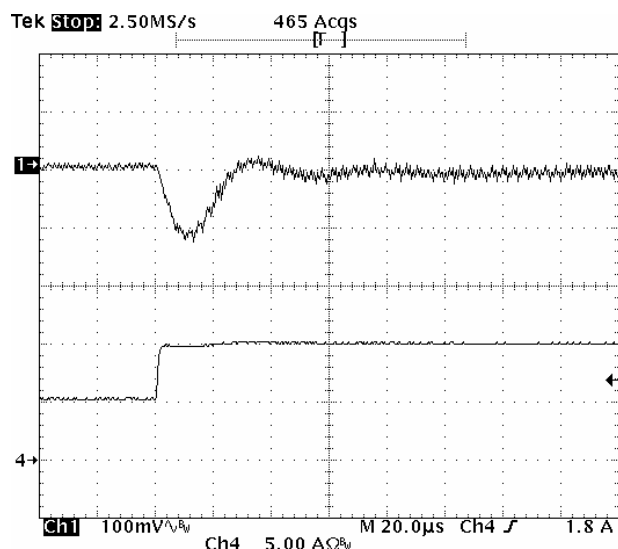
Fig-1.8V-6: Output voltage response for V_{out}=1.8V to positive load current step-change from 5A to 10A with slew rate of 5A/\mu s at V_{in}=5.0V . C_o=47\mu F \times 4 ceramic + 1\mu F ceramic.
