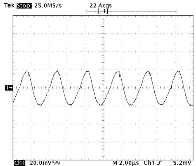
Fig-1.2V-5: Output voltage ripple (20mV/div.) for V_{out}=1.2V at full rated load current into a resistive load with external capacitance 47\mu F \times 4 ceramic + 1\mu F ceramic at V_{in}=5.0V .
