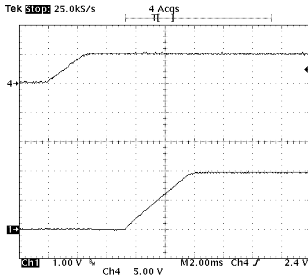
Fig-2.0V-4: Turn-on transient for V_{out}=2.0V with application of V_{in} at full rated load current (resistive) and 47\mu F \times 4 external capacitance at V_{in}=5.0V .
