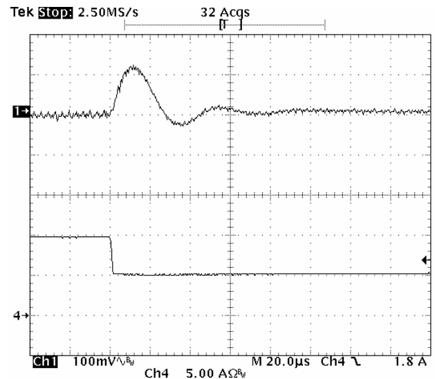
Fig-1.5V-7: Output voltage response for V_{out}=1.5V to positive load current step-change from 10A to 5A with slew rate of -5A/\mu s at V_{in}=5.0V . C_o=47\mu F \times 4 ceramic + 1\mu F ceramic.
