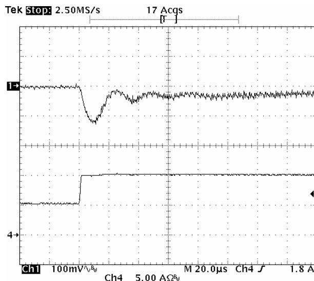
Fig-3.3V-6: Output voltage response for V_{out}=3.3V to positive load current step-change from 5A to 10A with slew rate of 5A/\mu s at V_{in}=5.0V . C_o=47\mu F \times 4 ceramic + 1\mu F ceramic.
