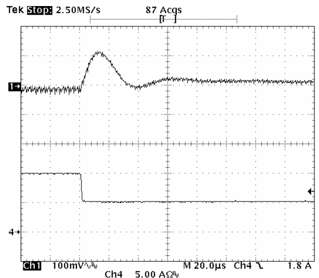
Fig-0.7525V-7: Output voltage response for V_{out}=0.7525V to positive load current step-change from 10A to 5A with slew rate of -5A/\mu s at V_{in}=5.0V . C_o=47\mu F \times 4 ceramic + 1\mu F ceramic.
