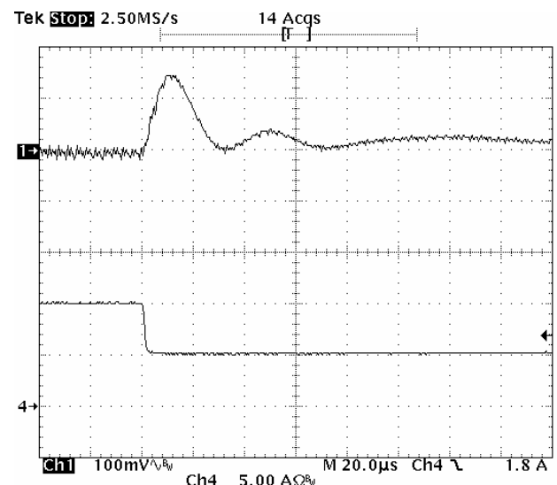
Fig-3.3V-7: Output voltage response for V_{out}=3.3V to positive load current step-change from 10A to 5A with slew rate of -5A/\mu s at V_{in}=5.0V . C_o=47\mu F \times 4 ceramic + 1\mu F ceramic.
