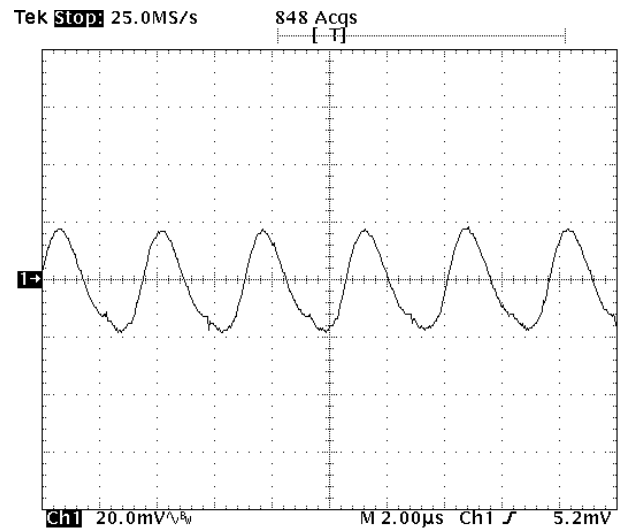
Fig-3.3V-5: Output voltage ripple (20mV/div.) for V_{out}=3.3V at full rated load current into a resistive load with external capacitance 47\mu F \times 4 ceramic + 1\mu F ceramic at V_{in}=5.0V .
