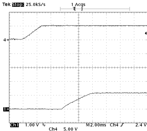
Fig-1.2V-4: Turn-on transient for V_{out}=1.2V with application of V_{in} at full rated load current (resistive) and 47\mu F \times 4 external capacitance at V_{in}=5.0V .
