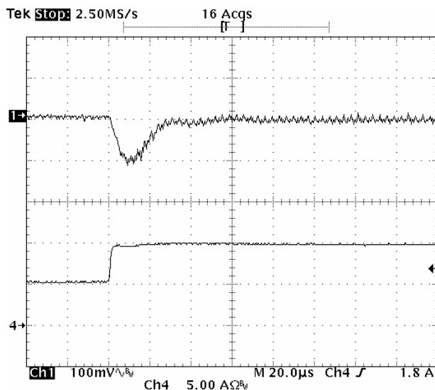
Fig-1.5V-6: Output voltage response for V_{out}=1.5V to positive load current step-change from 5A to 10A with slew rate of 5A/\mu s at V_{in}=5.0V . C_o=47\mu F \times 4 ceramic + 1\mu F ceramic.
