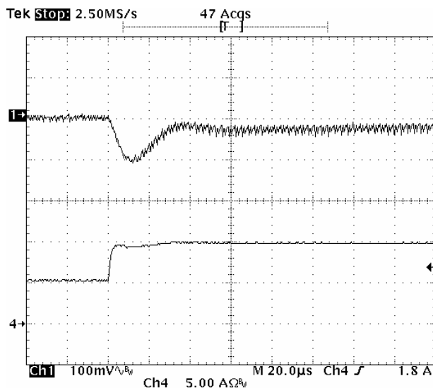
Fig-0.7525V-6: Output voltage response for V_{out}=0.7525V to positive load current step-change from 5A to 10A with slew rate of 5A/\mu s at V_{in}=5.0V . C_o=47\mu F \times 4 ceramic + 1\mu F ceramic.
