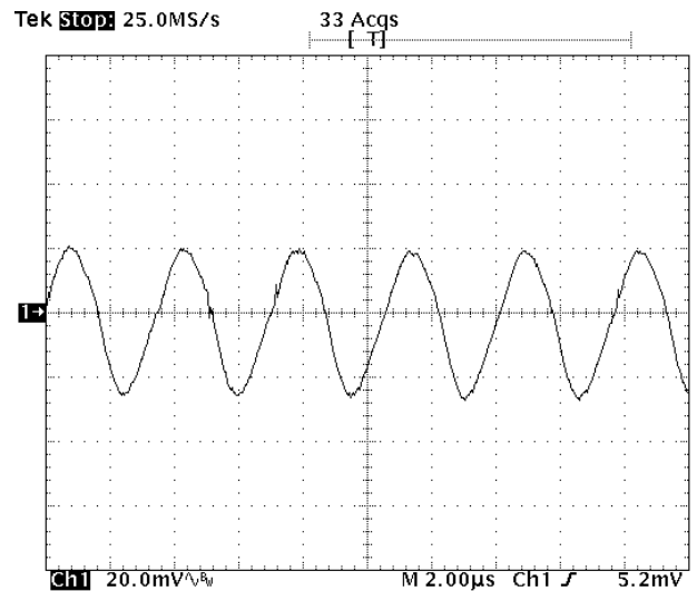
Fig-1.8V-5: Output voltage ripple (20mV/div.) for V_{out}=1.8V at full rated load current into a resistive load with external capacitance 47\mu F \times 4 ceramic + 1\mu F ceramic at V_{in}=5.0V .
