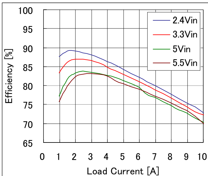
Fig-0.7255V-2: Efficiency vs. load current and input voltage for V_{out}=0.7525V . Airflow rate=200 LFM (1.0m/s) and T_a=25^{\circ}C .
