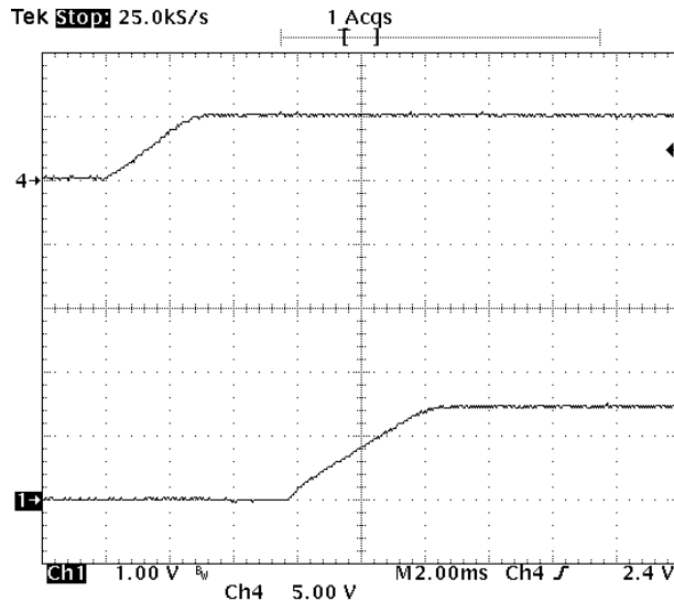
Fig-1.5V-4: Turn-on transient for V_{out}=1.5V with application of V_{in} at full rated load current (resistive) and 47\mu F \times 4 external capacitance at V_{in}=5.0V .
