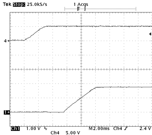
Fig-1.8V-4: Turn-on transient for V_{out}=1.8V with application of V_{in} at full rated load current (resistive) and 47\mu F \times 4 external capacitance at V_{in}=5.0V .
