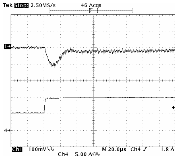
Fig-1.2V-6: Output voltage response for V_{out}=1.2V to positive load current step-change from 5A to 10A with slew rate of 5A/\mu s at V_{in}=5.0V . C_o=47\mu F \times 4 ceramic + 1\mu F ceramic.
