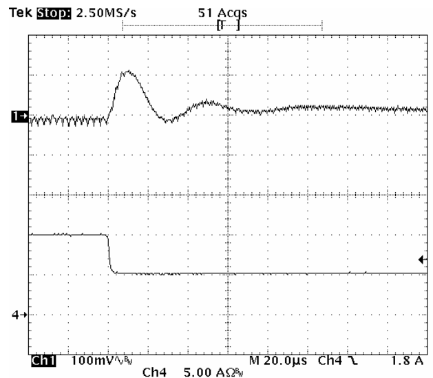
Fig-2.5V-7: Output voltage response for V_{out}=2.5V to positive load current step-change from 10A to 5A with slew rate of -5A/\mu s at V_{in}=5.0V . C_o=47\mu F \times 4 ceramic + 1\mu F ceramic.
