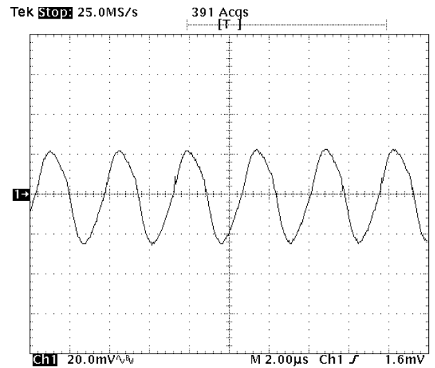
Fig-2.0V-5: Output voltage ripple (20mV/div.) for V_{out}=2.0V at full rated load current into a resistive load with external capacitance 47\mu F \times 4 ceramic + 1\mu F ceramic at V_{in}=5.0V .
