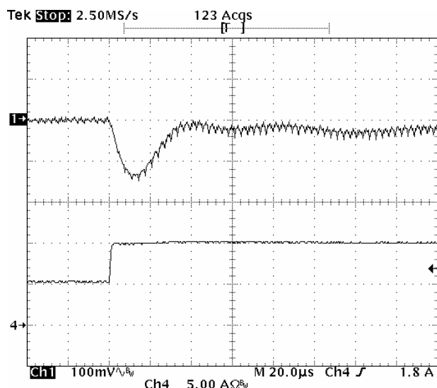
Fig-2.5V-6: Output voltage response for V_{out}=2.5V to positive load current step-change from 5A to 10A with slew rate of 5A/\mu s at V_{in}=5.0V . C_o=47\mu F \times 4 ceramic + 1\mu F ceramic.
