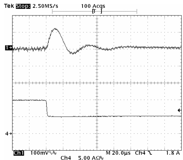
Fig-2.0V-7: Output voltage response for V_{out}=2.0V to positive load current step-change from 10A to 5A with slew rate of -5A/\mu s at V_{in}=5.0V . C_o=47\mu F \times 4 ceramic + 1\mu F ceramic.
