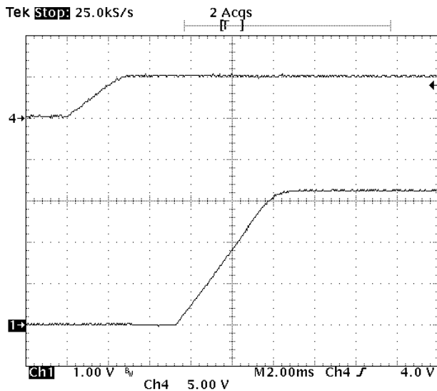
Fig-3.3V-4: Turn-on transient for V_{out}=3.3V with application of V_{in} at full rated load current (resistive) and 47\mu F \times 4 external capacitance at V_{in}=5.0V .
