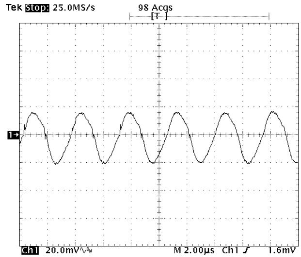
Fig-2.0V-5: Output voltage ripple (20mV/div.) for V_{out}=2.0V at full rated load current into a resistive load with external capacitance 47\mu F \times 2 ceramic + 1µF ceramic at V_{in}=5.0V . Time scale: 2µs/div
