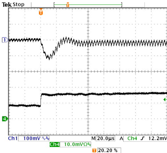
Fig-1.8V-6: Output voltage response for V_{out}=1.8V to positive load current step-change from 4A to 8A with slew rate of 5A/\mu s at V_{in}=5.0V . C_o=47\mu F \times 2 ceramic + 1\mu F ceramic.
