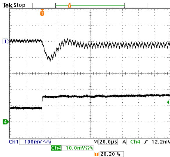
Fig-2.0V-6: Output voltage response for V_{out}=2.0V to positive load current step-change from 4A to 8A with slew rate of 5A/\mu s at V_{in}=5.0V . C_o=47\mu F \times 2 ceramic + 1µF ceramic. Top trace: output voltage (100mV/div.) Bottom trace: load current (5A/div.) Time scale: 20µs/div.
