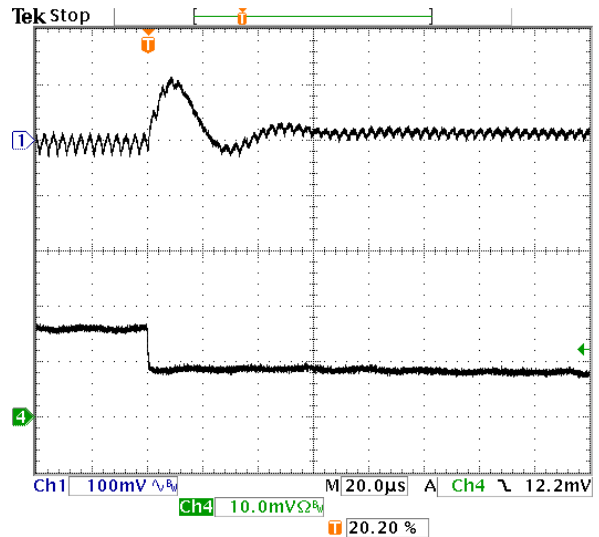
Fig-1.8V-7: Output voltage response for V_{out}=1.8V to positive load current step-change from 8A to 4A with slew rate of -5A/\mu s at V_{in}=5.0V . C_o=47\mu F \times 2 ceramic + 1\mu F ceramic.
