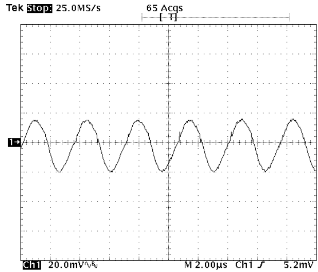
Fig-1.8V-5: Output voltage ripple (20mV/div.) for V_{out}=1.8V at full rated load current into a resistive load with external capacitance 47\mu F \times 2 ceramic + 1\mu F ceramic at V_{in}=5.0V .
