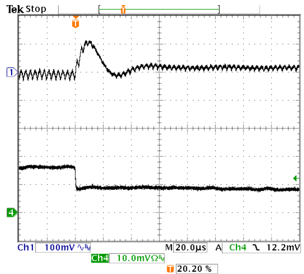
Fig-2.0V-7: Output voltage response for V_{out}=2.0V to positive load current step-change from 8A to 4A with slew rate of -5A/\mu s at V_{in}=5.0V . C_o=47\mu F \times 2 ceramic + 1µF ceramic. Top trace: output voltage (100mV/div.) Bottom trace: load current (5A/div.) Time scale: 20µs/div.
