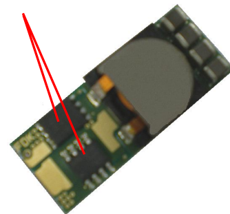
Fig. D: Location of the thermocouples for thermal testing
