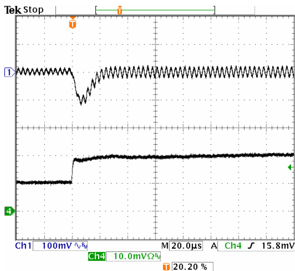
Fig-1.2V-6: Output voltage response for V_{out}=1.2V to positive load current step-change from 5A to 10A with slew rate of 5A/\mu s at V_{in}=5.0V . C_o=47\mu F \times 2 ceramic.
