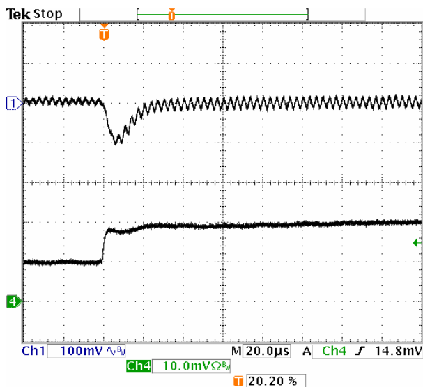
Fig-0.7525V-6: Output voltage response for Vout=0.7525V to positive load current step-change from 5A to 10A with slew rate of 5A/ \mu s at Vin=5.0V. Co=47 \mu Fx2 ceramic.
