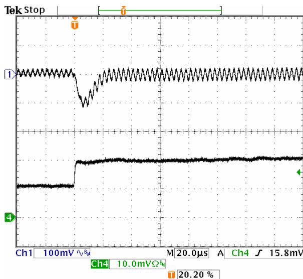
Fig-1.5V-6: Output voltage response for V_{out}=1.5V to positive load current step-change from 5A to 10A with slew rate of 5A/\mu s at V_{in}=5.0V . C_o=47\mu F \times 2 ceramic.
