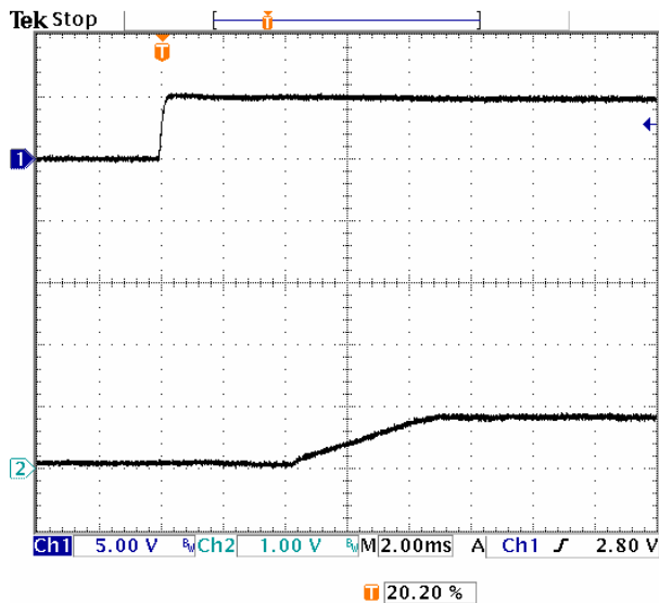
Fig-0.7525V-4: Turn-on transient for Vout=0.7525V with application of Vin at full rated load current (resistive) and 47 \mu Fx2 external capacitance at Vin=5.0V.
