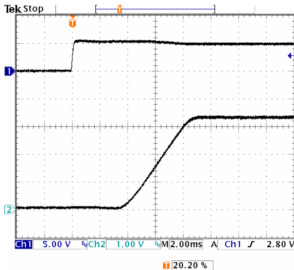
Fig-3.3V-4: Turn-on transient for V_{out}=3.3V with application of V_{in} at full rated load current (resistive) and 47\mu F \times 2 external capacitance at V_{in}=5.0V .
