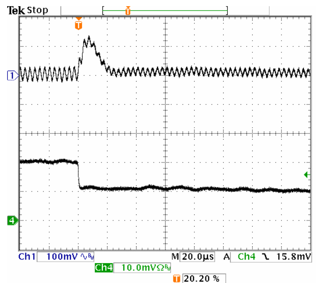
Fig-1.8V-7: Output voltage response for V_{out}=1.8V to positive load current step-change from 10A to 5A with slew rate of -5A/\mu s at V_{in}=5.0V . C_o=47\mu F \times 2 ceramic.
