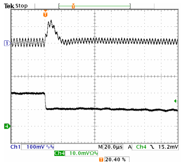
Fig-2.5V-7: Output voltage response for V_{out}=2.5V to positive load current step-change from 10A to 5A with slew rate of -5A/\mu s at V_{in}=5.0V . C_o=47\mu F \times 2 ceramic.
