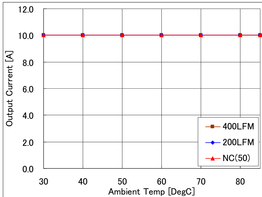
Fig-1.5V-1: Available load current vs. ambient temperature and airflow rates for V_{out}=1.5V with V_{in}=5.0V . Maximum component temperature \leq 120^{\circ}C
