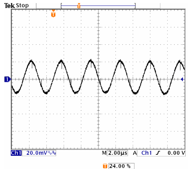
Fig-3.3V-5: Output voltage ripple (20mV/div.) for V_{out}=3.3V at full rated load current into a resistive load with external capacitance 47\mu F \times 2 ceramic + 1\mu F ceramic at V_{in}=5.0V .
