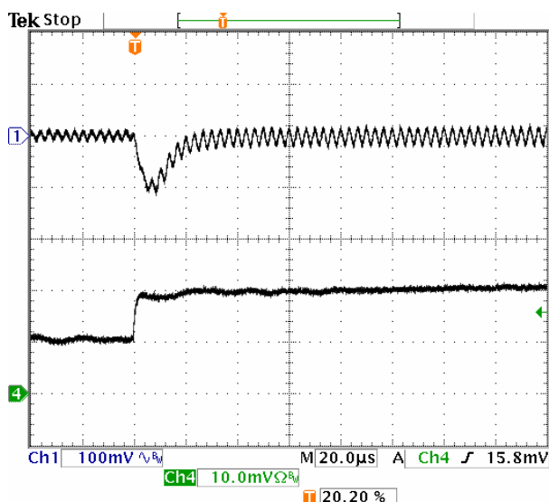
Fig-1.0V-6: Output voltage response for V_{out}=1.0V to positive load current step-change from 5A to 10A with slew rate of 5A/\mu s at V_{in}=5.0V . C_o=47\mu F \times 2 ceramic.
