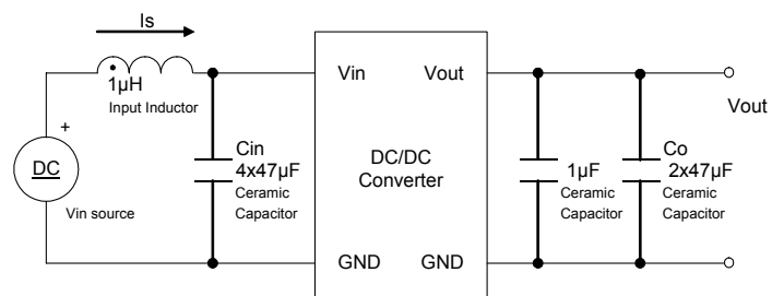
Fig. H: Test setup for measuring input reflected ripple current
