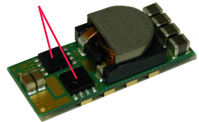
Thermocouple
