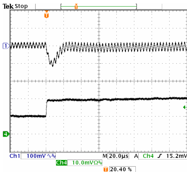
Fig-2.5V-6: Output voltage response for V_{out}=2.5V to positive load current step-change from 5A to 10A with slew rate of 5A/\mu s at V_{in}=5.0V . C_o=47\mu F \times 2 ceramic.
