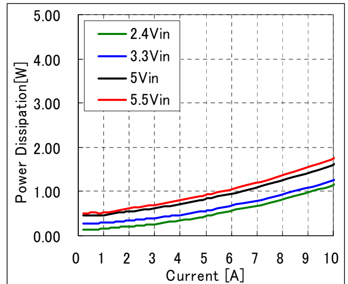
Fig-1.5V-3: Power dissipation vs. load current and input voltage for V_{out}=1.5V . Airflow rate=200 LFM (1.0m/s) and T_a=25^{\circ}C .
