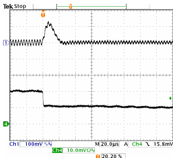
Fig-1.0V-7: Output voltage response for V_{out}=1.0V to positive load current step-change from 10A to 5A with slew rate of -5A/\mu s at V_{in}=5.0V . C_o=47\mu F \times 2 ceramic.
