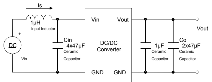
Fig. G: Test setup for measuring output voltage ripple
