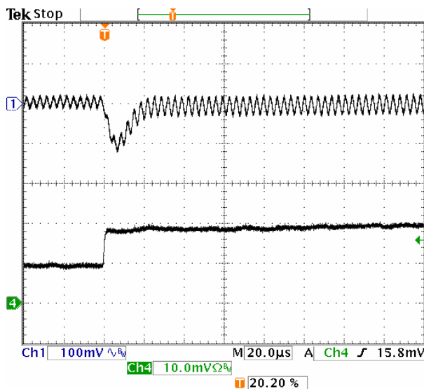
Fig-2.0V-6: Output voltage response for V_{out}=2.0V to positive load current step-change from 5A to 10A with slew rate of 5A/\mu s at V_{in}=5.0V . C_o=47\mu F \times 2 ceramic.
