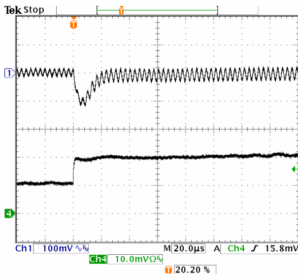
Fig-1.8V-6: Output voltage response for V_{out}=1.8V to positive load current step-change from 5A to 10A with slew rate of 5A/\mu s at V_{in}=5.0V . C_o=47\mu F \times 2 ceramic.
