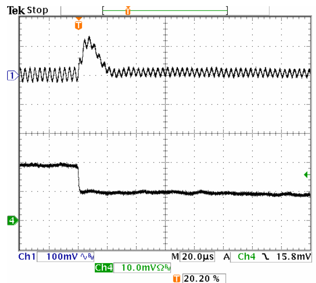
Fig-2.0V-7: Output voltage response for V_{out}=2.0V to positive load current step-change from 10A to 5A with slew rate of -5A/\mu s at V_{in}=5.0V . C_o=47\mu F \times 2 ceramic.
