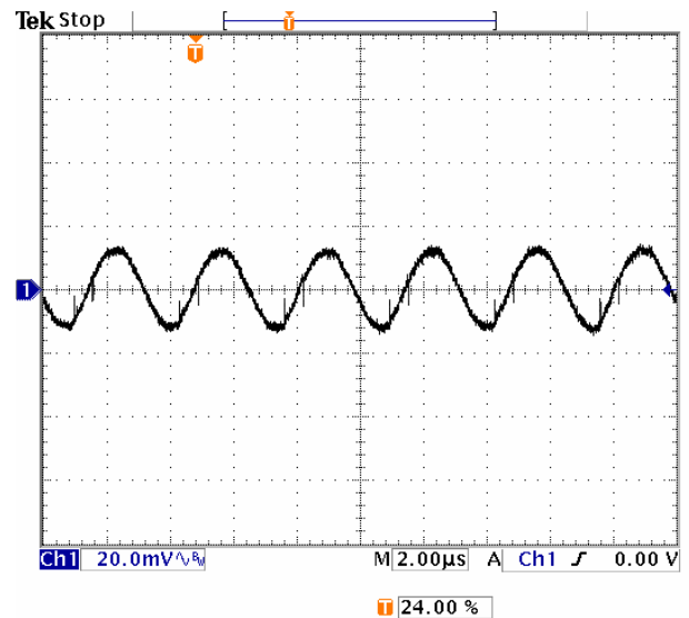
Fig-0.7255V-5: Output voltage ripple (20mV/div.) for Vout=0.7525V at full rated load current into a resistive load with external capacitance 47 \mu Fx2 ceramic + 1 \mu F ceramic at Vin=5.0V.
