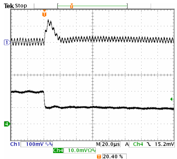
Fig-3.3V-7: Output voltage response for V_{out}=3.3V to negative load current step-change from 10A to 5A with slew rate of -5A/\mu s at V_{in}=5.0V . C_o=47\mu F \times 2 ceramic.
