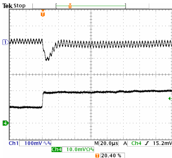
Fig-3.3V-6: Output voltage response for V_{out}=3.3V to positive load current step-change from 5A to 10A with slew rate of 5A/\mu s at V_{in}=5.0V . C_o=47\mu F \times 2 ceramic.
