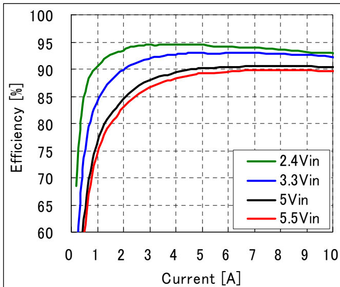
Fig-1.5V-2: Efficiency vs. load current and input voltage for V_{out}=1.5V . Airflow rate=200 LFM (1.0m/s) and T_a=25^{\circ}C .
