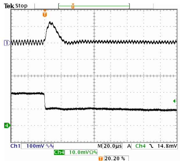
Fig-0.7525V-7: Output voltage response for Vout=0.7525V to positive load current step-change from 10A to 5A with slew rate of -5A/ \mu s at Vin=5.0V. Co=47 \mu Fx2 ceramic.
