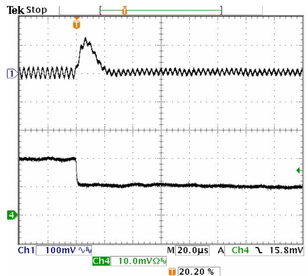
Fig-1.2V-7: Output voltage response for V_{out}=1.2V to positive load current step-change from 10A to 5A with slew rate of -5A/\mu s at V_{in}=5.0V . C_o=47\mu F \times 2 ceramic.
