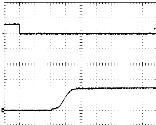
Fig.1.5V-5: Turn-on transient at full rated load current (resistive) plus 20,000 \mu F at Vin=48V, triggered via ON/OFF pin. Top trace: ON/OFF signal (5V/div). Bottom trace: output voltage (1V/div). Time scale: 2ms/div
