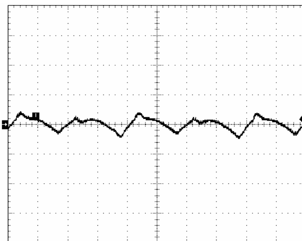
Fig.1.5V-7: Output voltage ripple (50mV/div) at full rated load current into a resistive load with Co=10 \mu F tantalum + 1 \mu F ceramic and Vin=48V. Time scale: 1 \mu s/div
