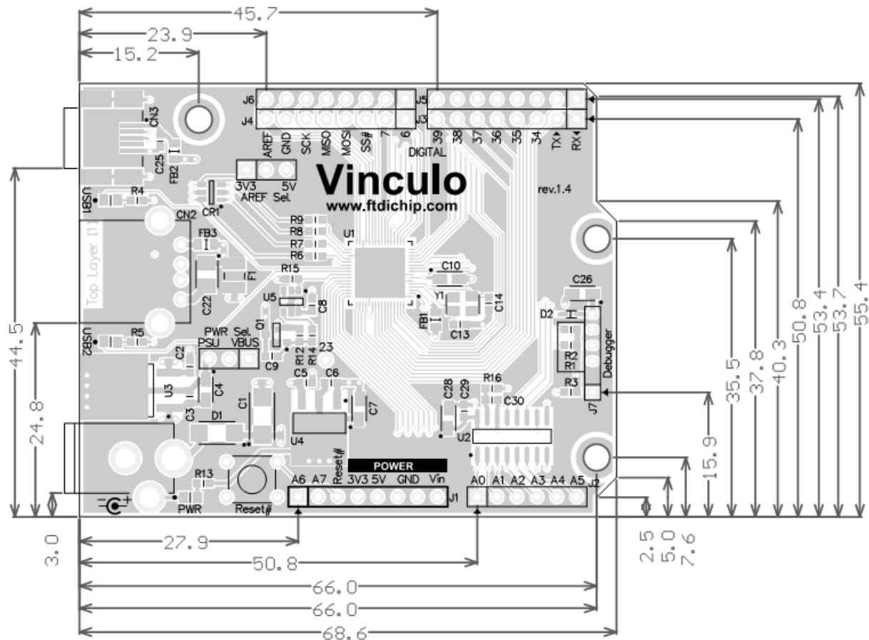
Figure 8.1 - Vinculo Dimensions
