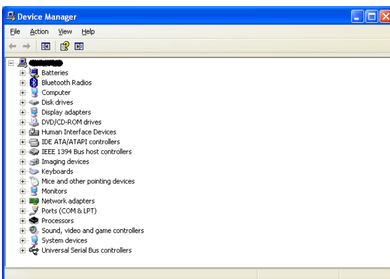
Figure 2.6 Device Manager
