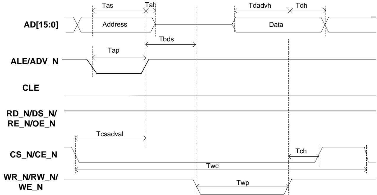
Figure 6-4 Write in NOR mode
