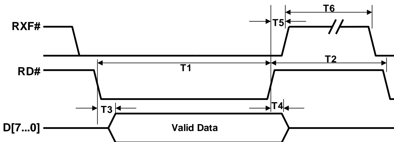
Figure 3.3 FIFO Read Cycle
