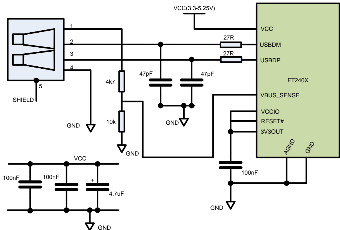
Figure 6.2 Self-Powered Configuration
