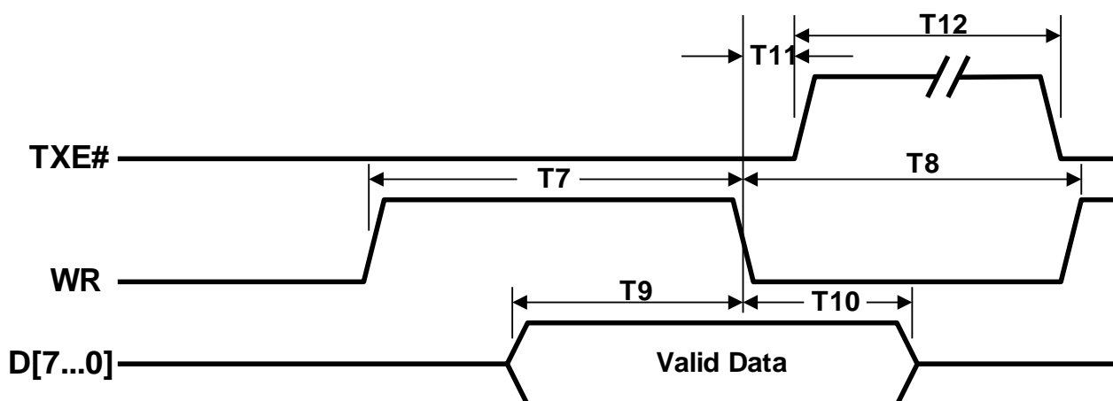
Figure 3.4 FIFO Write Cycle
