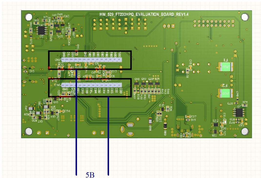
Figure 3 - UMFT233HPEV Evaluation Module Board – Bottom View
