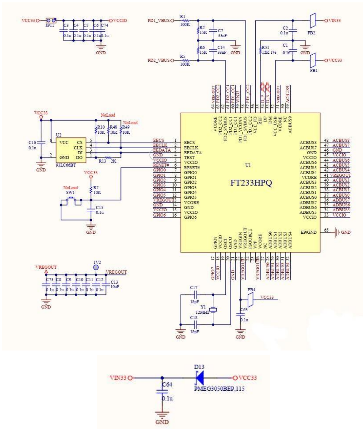
Figure 6 - FT233HPQ IC
