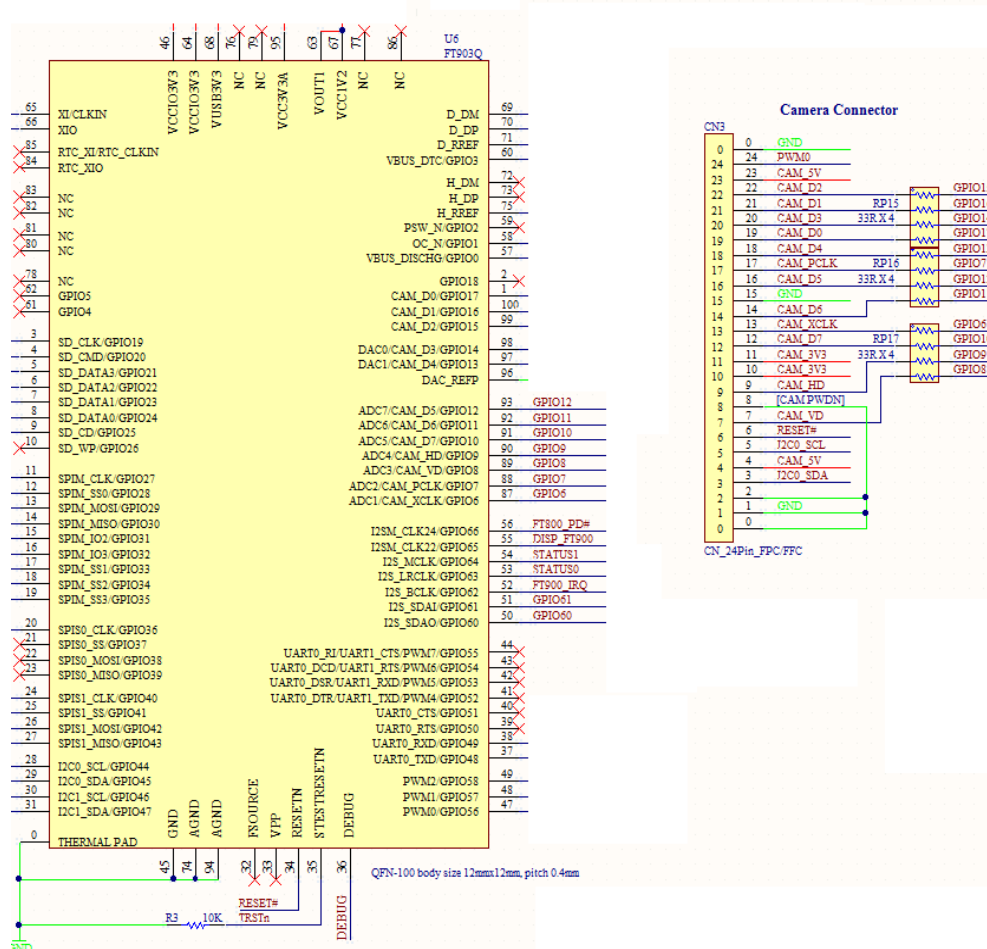
Figure 6 - Camera Interface
