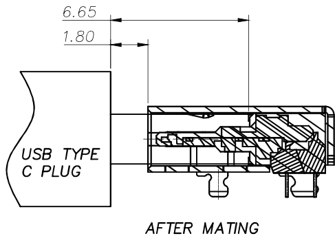
AFTER MATING
