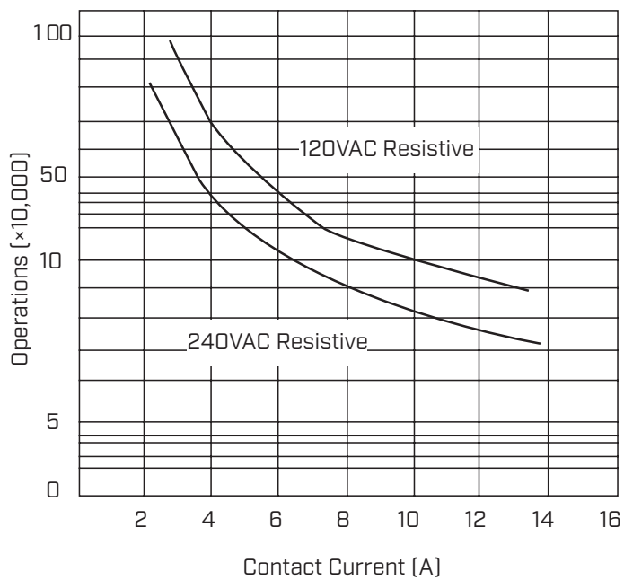
Life Curve
