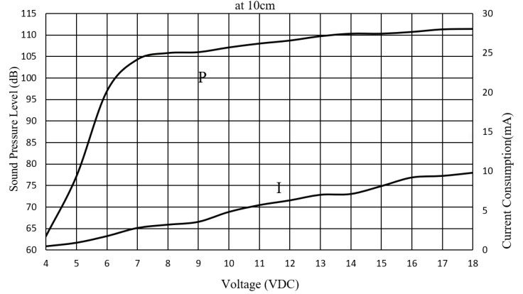
P: Voltage vs. Sound Pressure Level I: Voltage vs. Current Consumption [Slow Pulse Mode]
