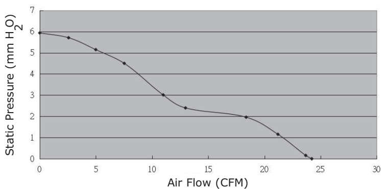
CFM-6015BF-255-375
