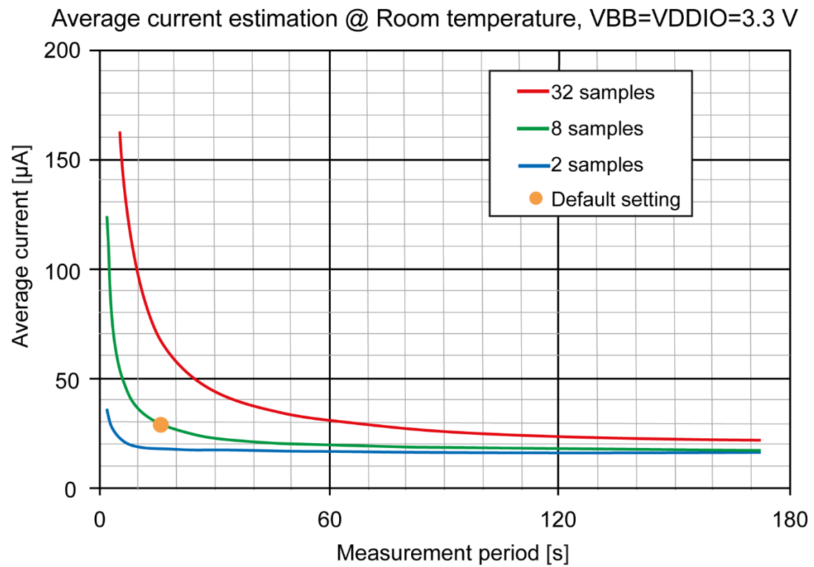
Figure 4 Average current
