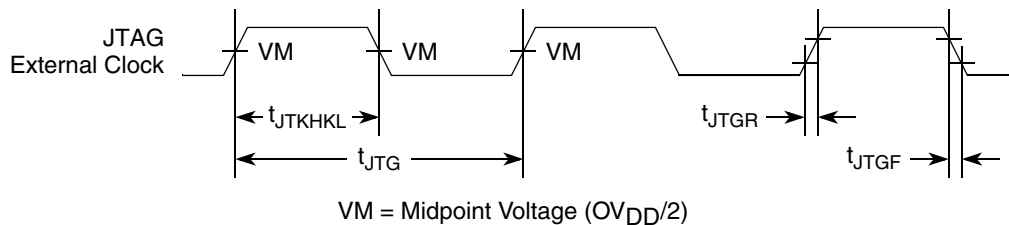
Figure 31. JTAG Clock Input Timing Diagram
