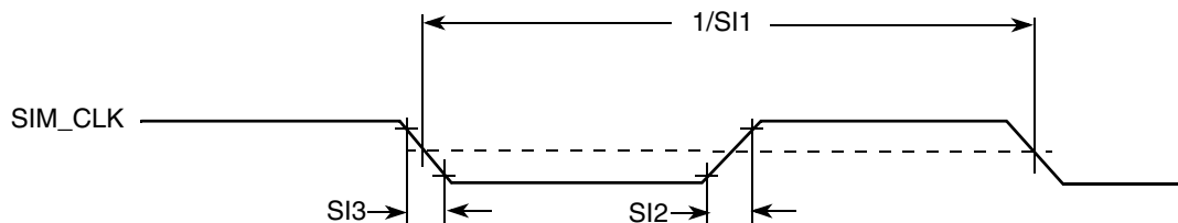
Figure 46. USIM Clock Timing Diagram
