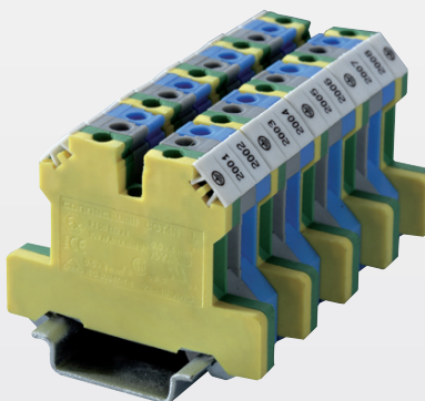
Assembly example for single phase 3 wire circuits.
