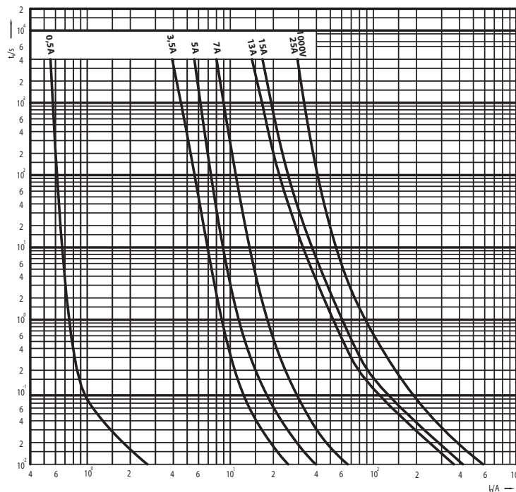
CH 10x38 gPV I/t characteristics
