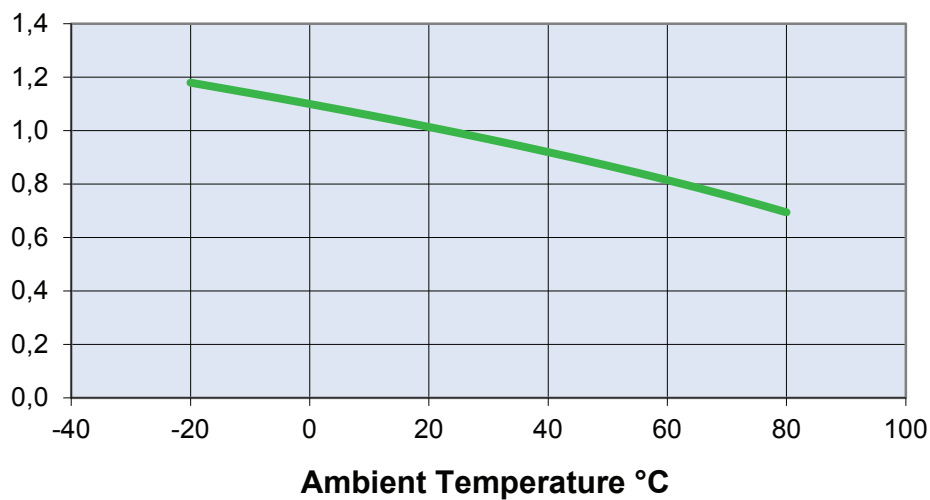
CH10x85 gPV Temperature Derating Factor
