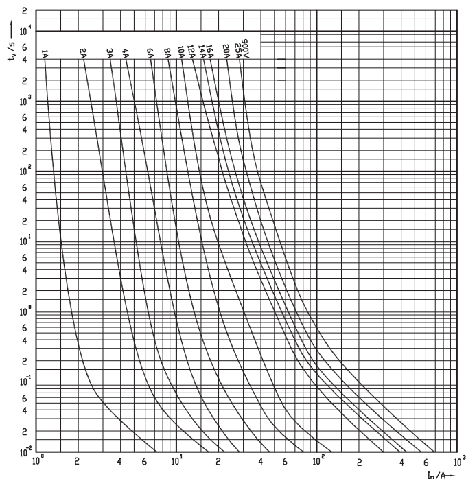
CH 10x38 gPV I/t characteristics
