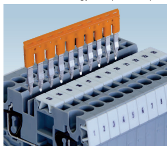
Push-In Technology Multipole Jumpers
