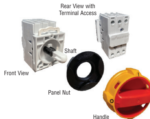
Assembly Example RT 340 L42LKX50YR
