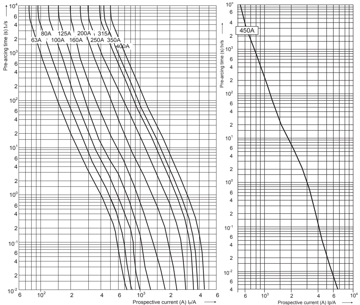
gPV 1100V t-I characteristics
