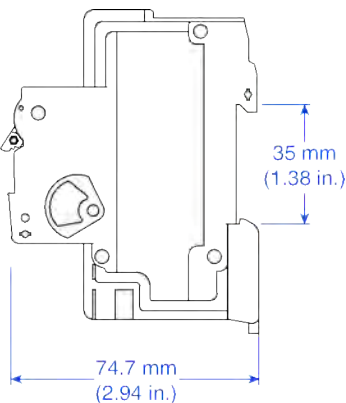
Dimensions in mm side view
