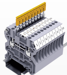
2 Jumper Channels
