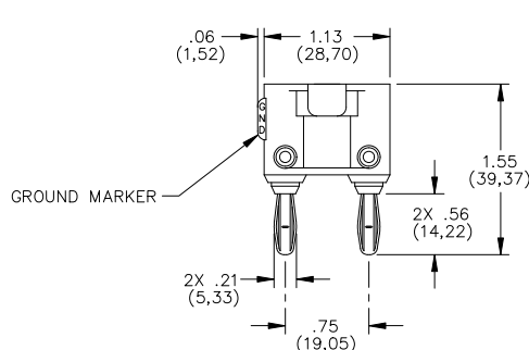
Model MDP-ST Double Banana Plug with Solder Turret Terminals
