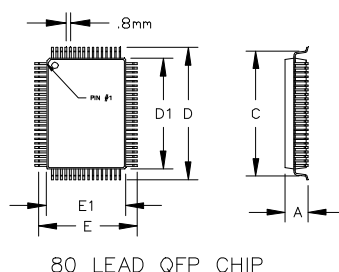
80 LEAD QFP CHIP
