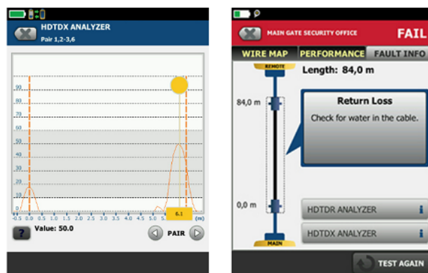
High Definition Time Domain Cross talk (HTDX) shows the far end connection is clearly the issue
