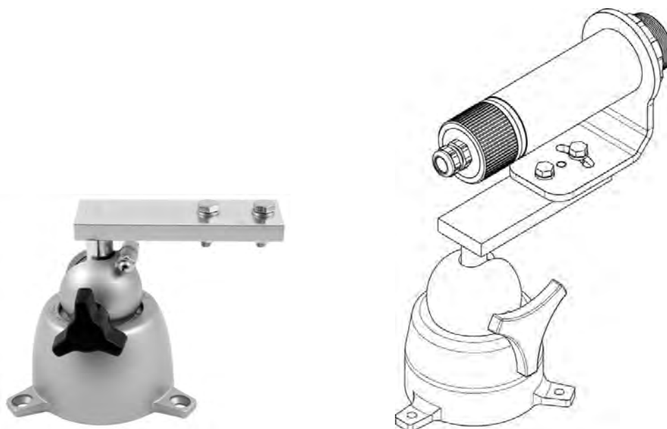
Figure 13-15: Swivel Bracket
