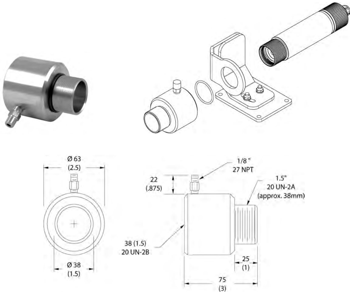
Figure 13-22: Air Purge
