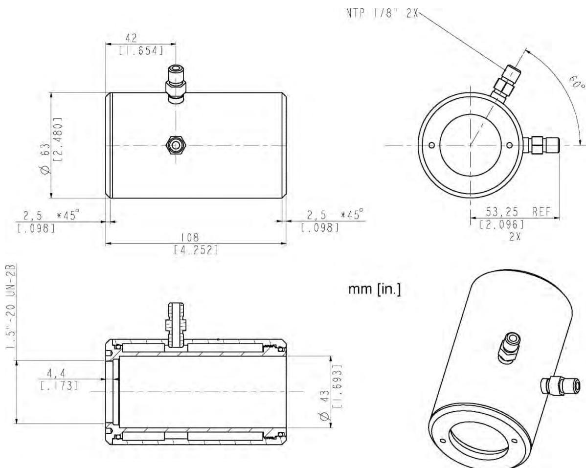
Figure 13-23: Air/Water-Cooled Housing
