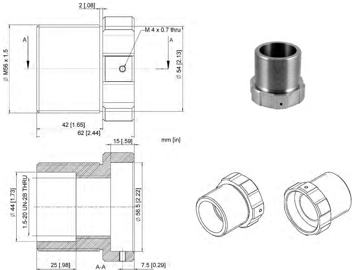
Figure 13-24: Thread Adapter
