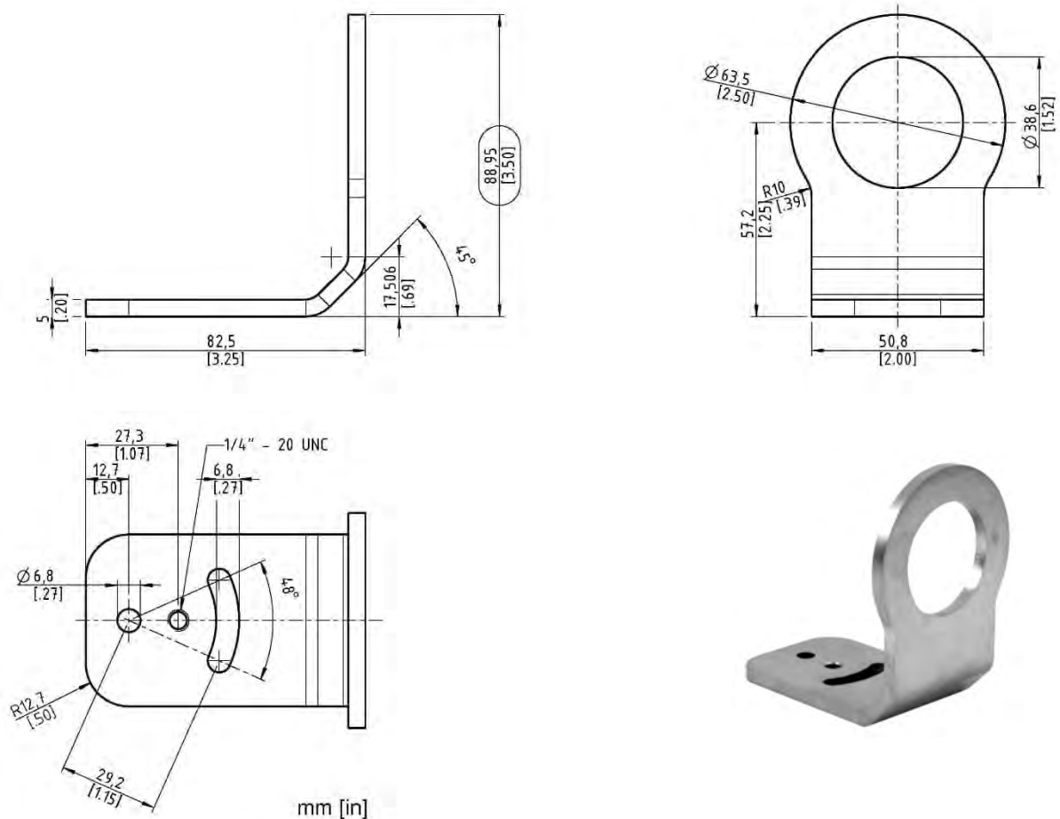
Figure 13-13: Fixed Bracket
