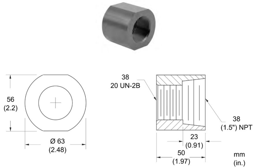
Figure 13-19: Pipe Adapter
