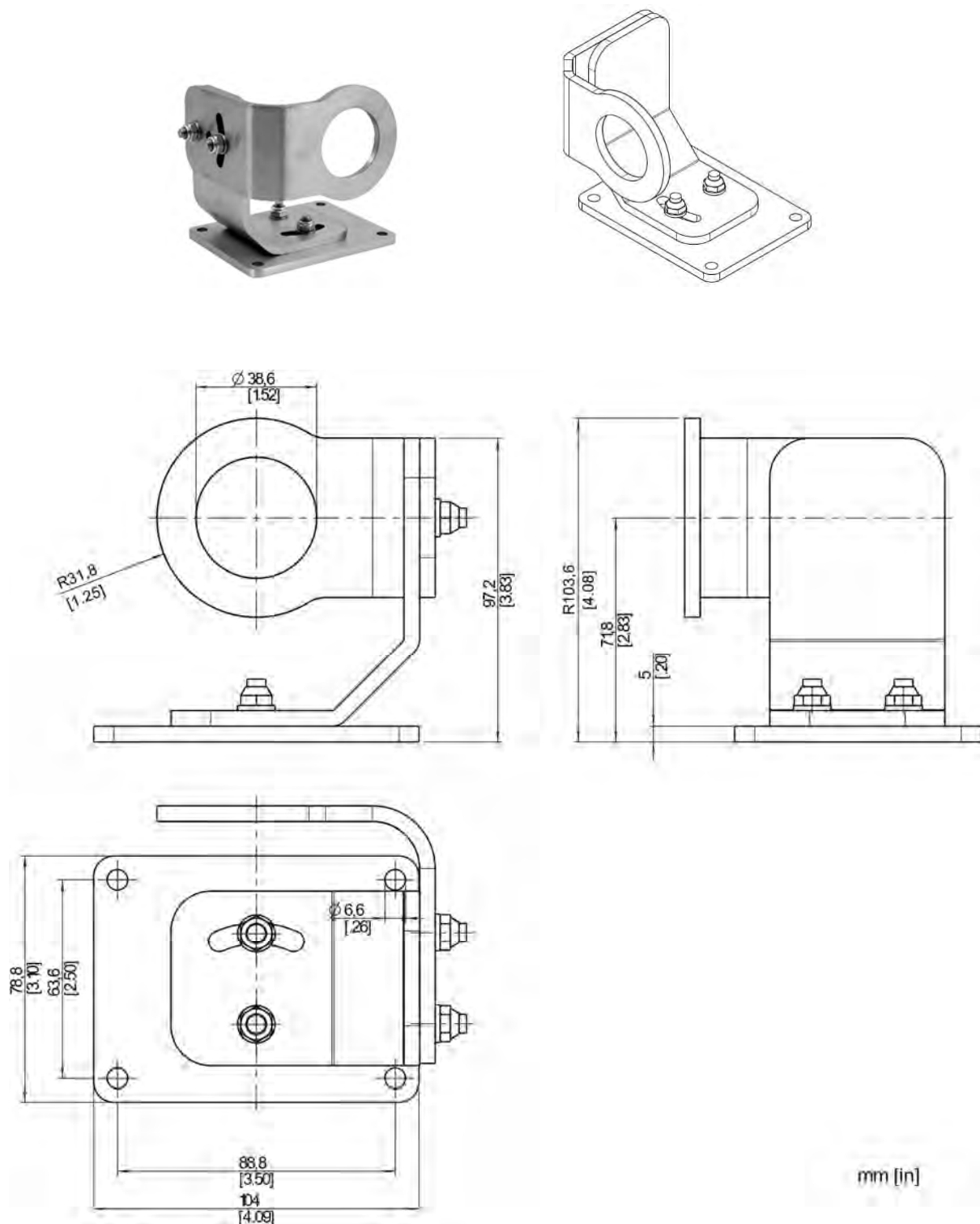
Figure 13-14: Adjustable Bracket
