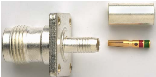
Model 7064 BNC (M) 50 Ω RG-58, 58A, 58C, 141, 303, LMR195, Belden 7806A.
