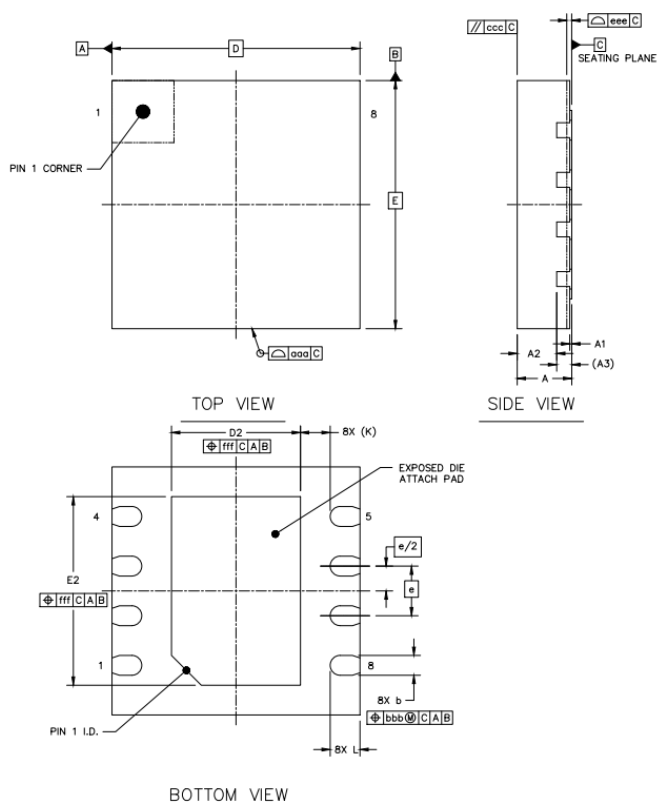
Figure 26 : DFN8 POD IN100-D1-R-YC1I
