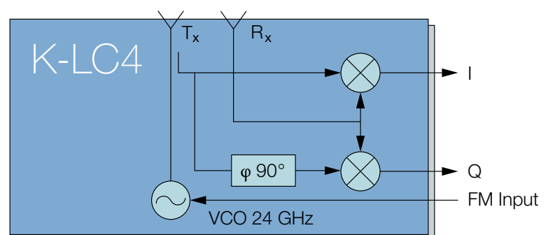
Figure 1: Blockdiagram
