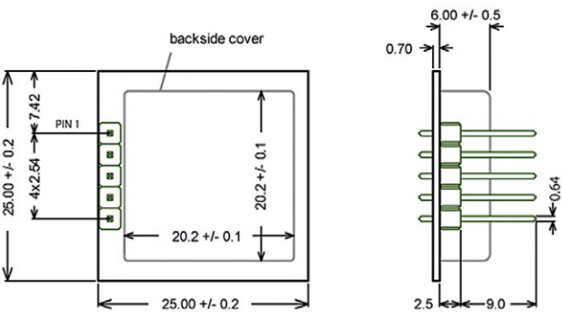
Figure 3: Mechanical data
