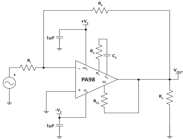
Figure 2: Typical Connections
