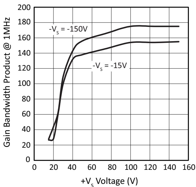
Figure 5: Gain Bandwidth vs. +Supply Voltage
