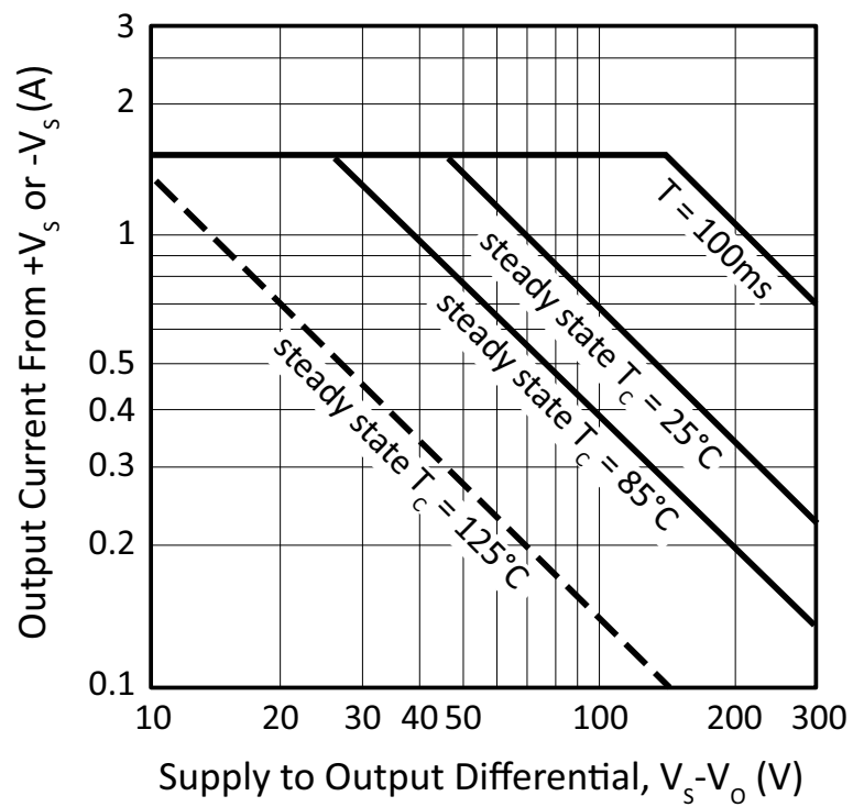
Figure 14: SOA
