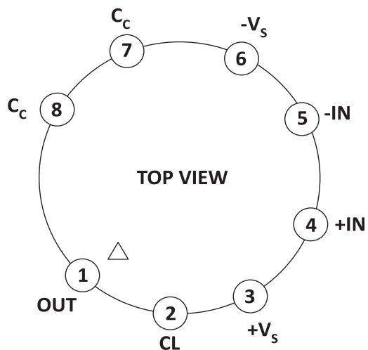
Figure 2: External Connections
