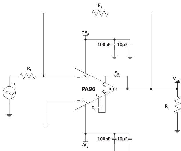
Figure 1: Typical Connection
