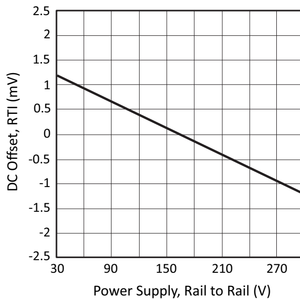
Figure 10: DC Offset vs. Power Supply
