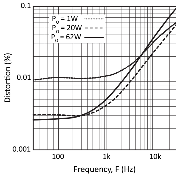
Figure 11: Harmonic Distortion
