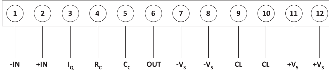
Figure 3: External Connections
