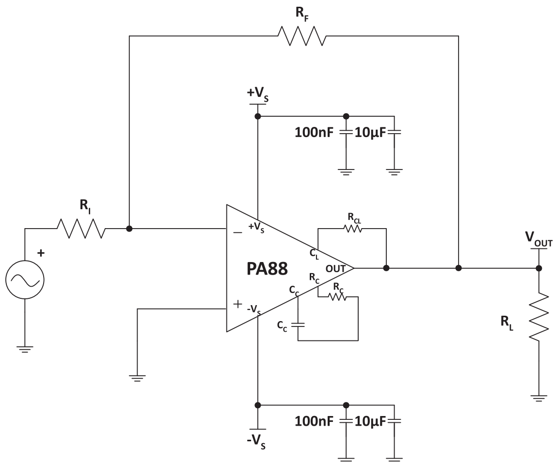
Figure 1: Typical Connection
