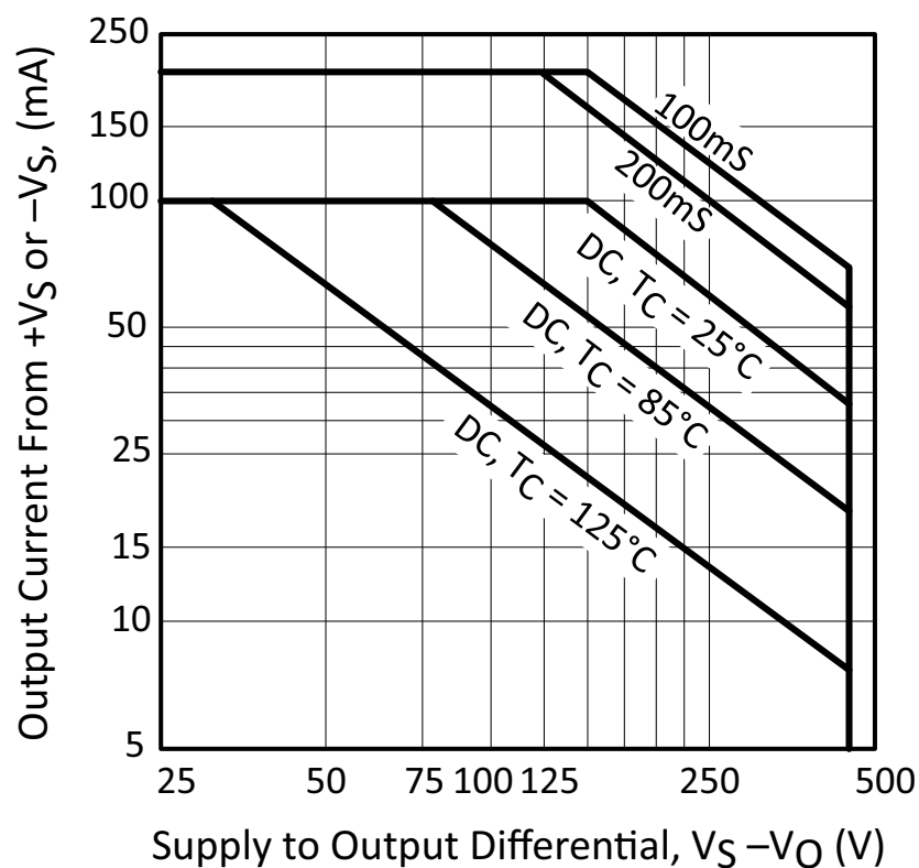
Figure 15: SOA
