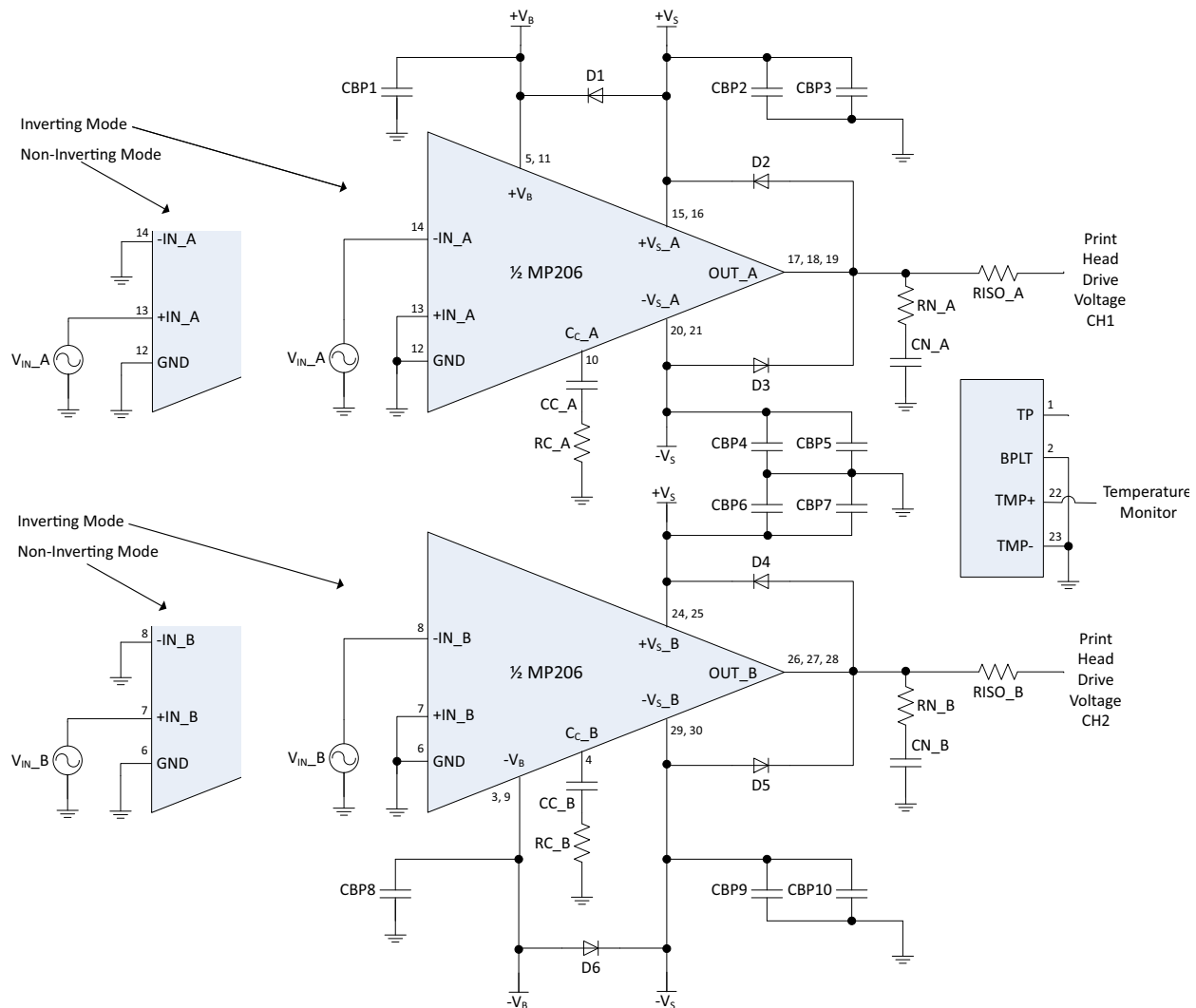
Figure 2: Typical Connection
