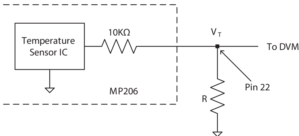
Figure 17: Temperature Sensor
