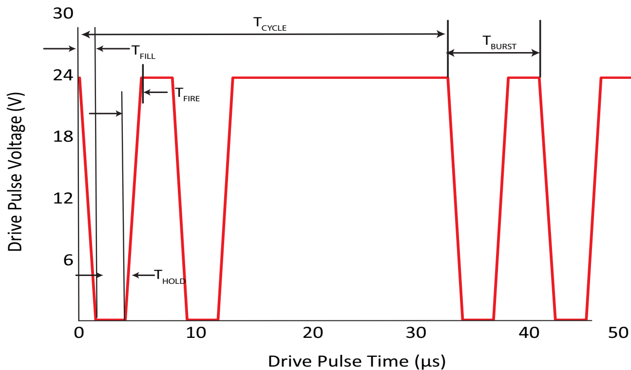
Figure 10: Example Waveform
