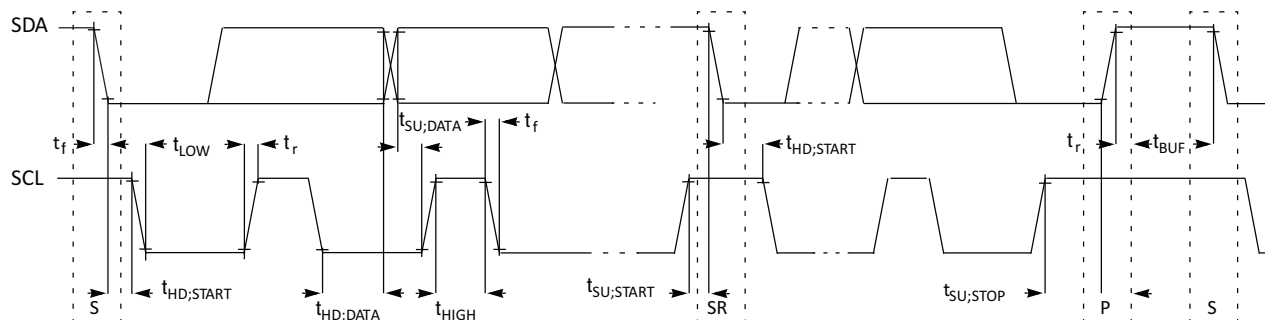
Figure 4: I2C Timing
