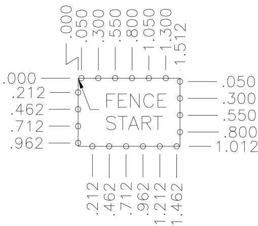
.25" Pin Pattern
