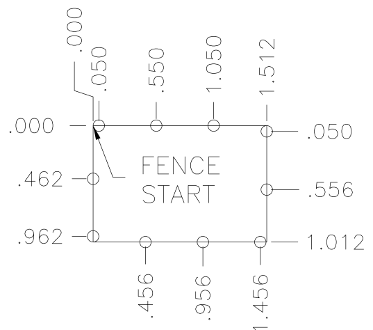
.50" Pin Pattern
